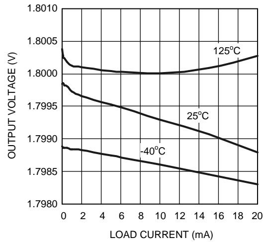
Figure 12. Load Regulation
