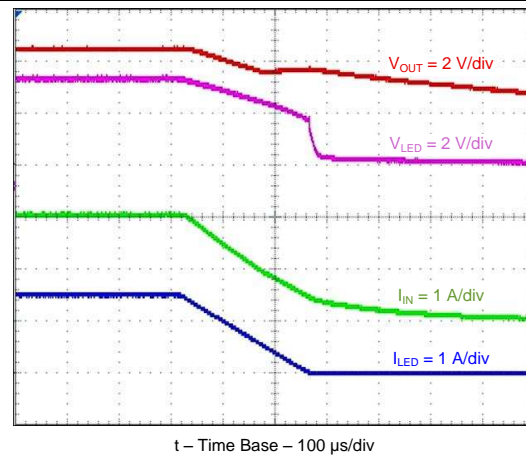
Figure 42. Flash Ramp-Down
