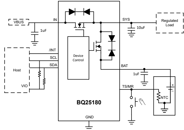
Simplified Schematic
