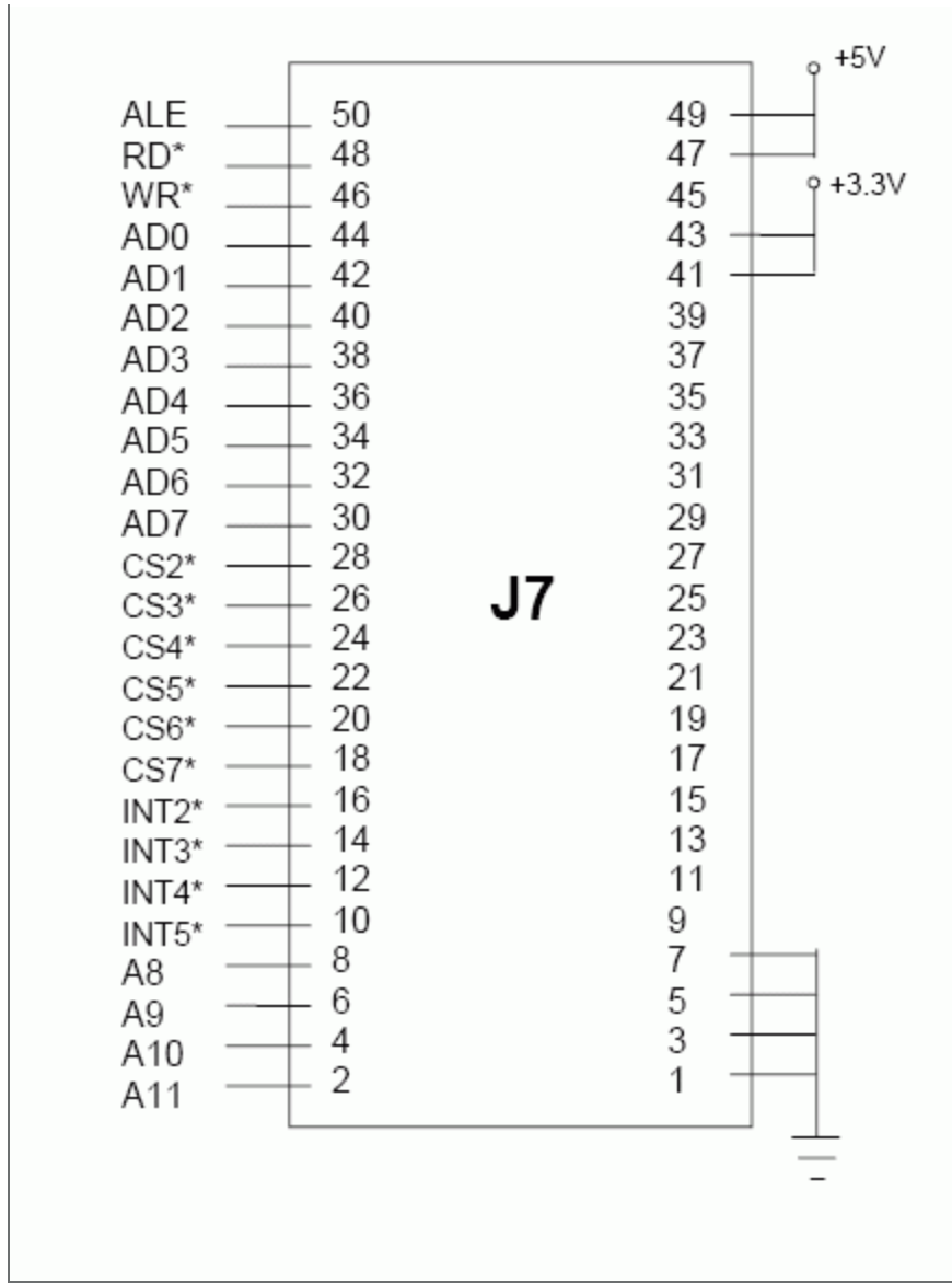
Figure 1. J7 Expansion Port. *denotes active-low signal.
